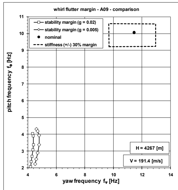
Fig. 5. Whirl flutter stability margin evaluation
