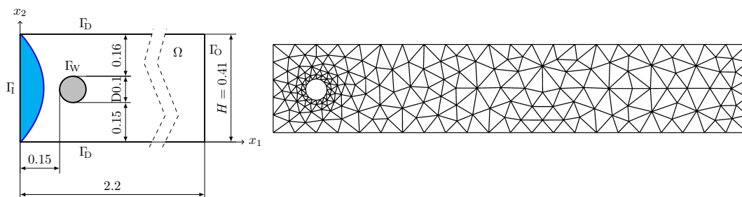
Fig. 1. (Left) Sketch of the computational domain. (Right) Computational grid consisting of 356 elements.
