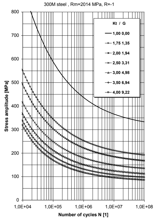
Fig. 3. Synthetic fatigue curves
