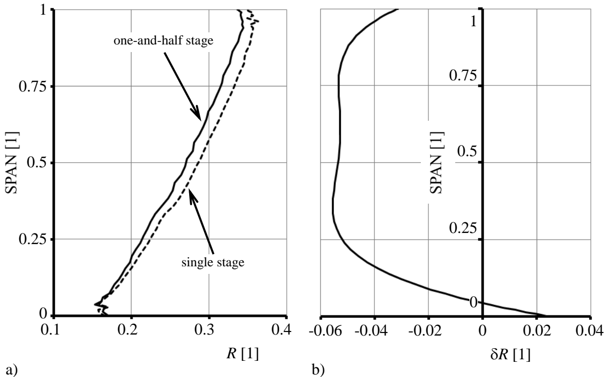
Fig. 2. Span wise distribution of the degree of reaction (a), relative change of the degree of reaction (b)
